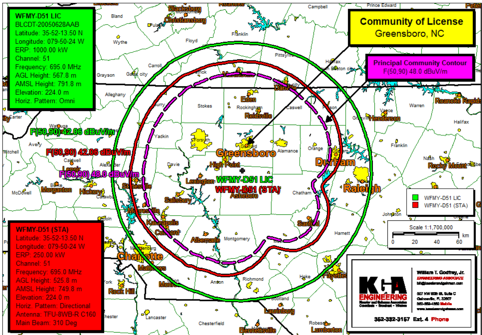
WFMY-D51 Pre-Auction LIC vs. WFMY-D51 Pre-Auction STA (TFU-8WB-R C160 @ 310 Degrees)
