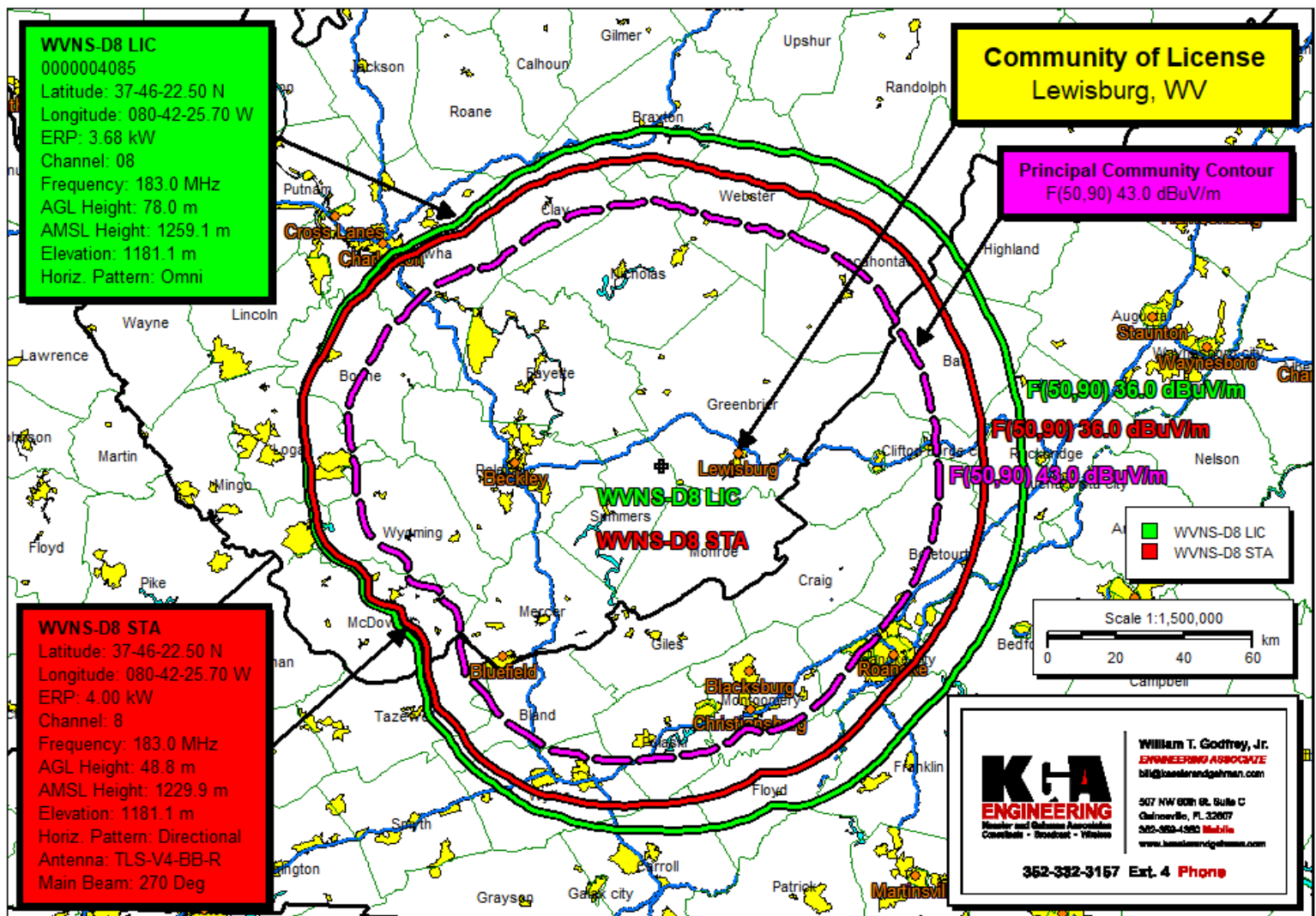
WVNS-D8 Pre-Auction LIC vs. WVNS-D8 Pre-Auction Interim (TLS-V4BB-R @ 270 Deg)
